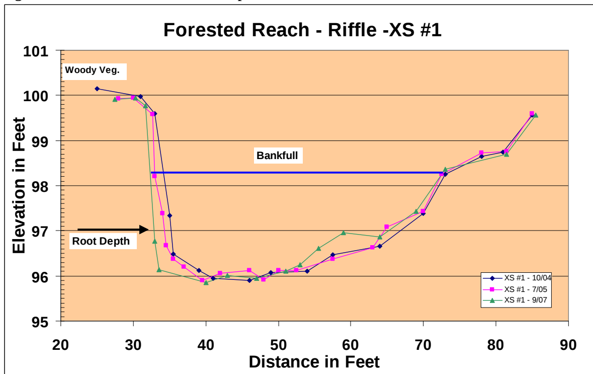
Figure A1-6. Riffle Cross-section in forested reach.
