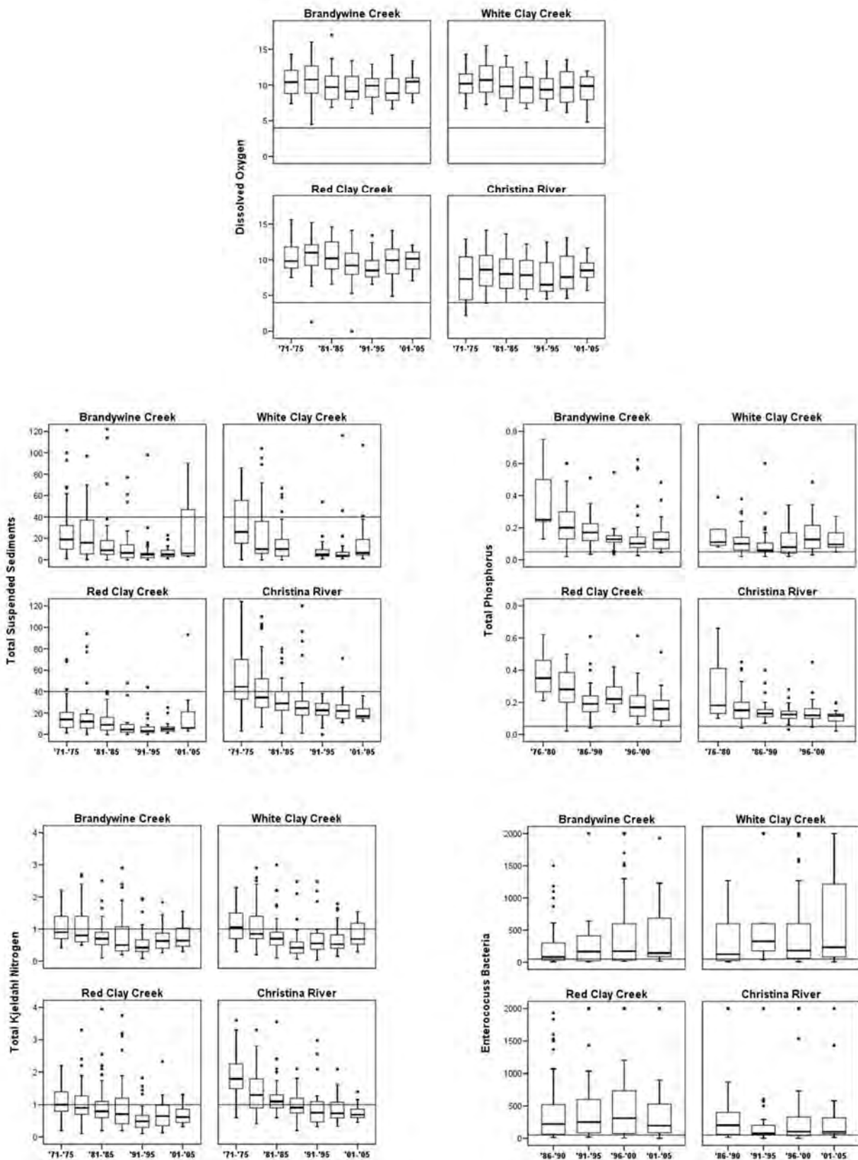
Figure 4.12. DO, TSS, TP, TN, and bacteria trends in the Christina Basin subwatersheds.
