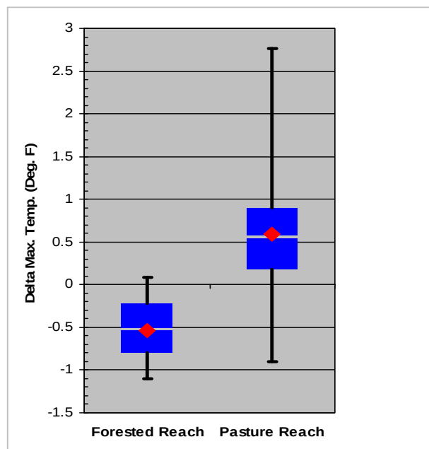
Figure 4.5. Mean daily delta maximum temperatures for forested and pasture stream reaches.
