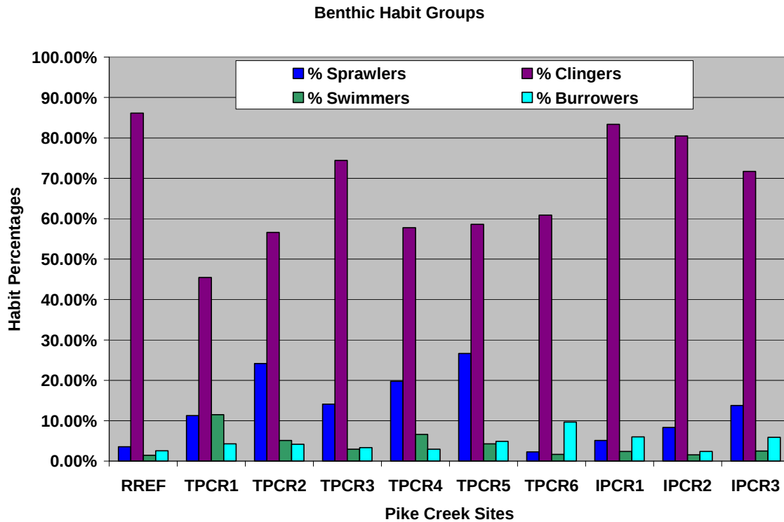
Figure 15. Percentages of Benthic Habit Groups for Pike Creek. Pike Creek is dominated by clingers. The 2006 restored sites are TPCR 1-6. The 2006 upstream, unrestored sites are IPCR 1-3. The 2006 regional reference is RREF.
