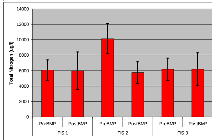
Figure Error! No text of specified style in document..1 Storm-flow Total Nitrogen, Fecal Coliform, and CBOD5 at FIS1, FIS2, and FIS3. Post-BMP mean total nitrogen concentration, fecal coliform numbers, and CBOD5 concentration are less than pre-BMP means at FIS2 (n= 4, one tailed t-test, p < 0.05 ).
