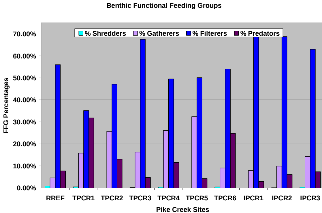
Figure 16. Percentages of Benthic Functional Feeding Groups (FFG). Pike Creek is dominated by filterers. Site RREF is the 2006 regional reference. Sites TPCR 1-6 are the 2006 restored sites. Sites IPCR 1-3 are the 2006 upstream, unrestored sites.
