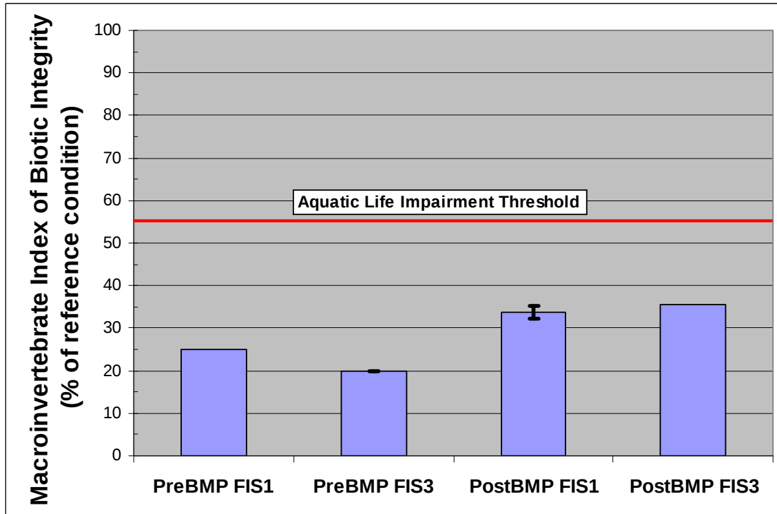
Figure 4.7. Macroinvertebrate IBI Scores on UNT W.Branch Brandywine Creek.
