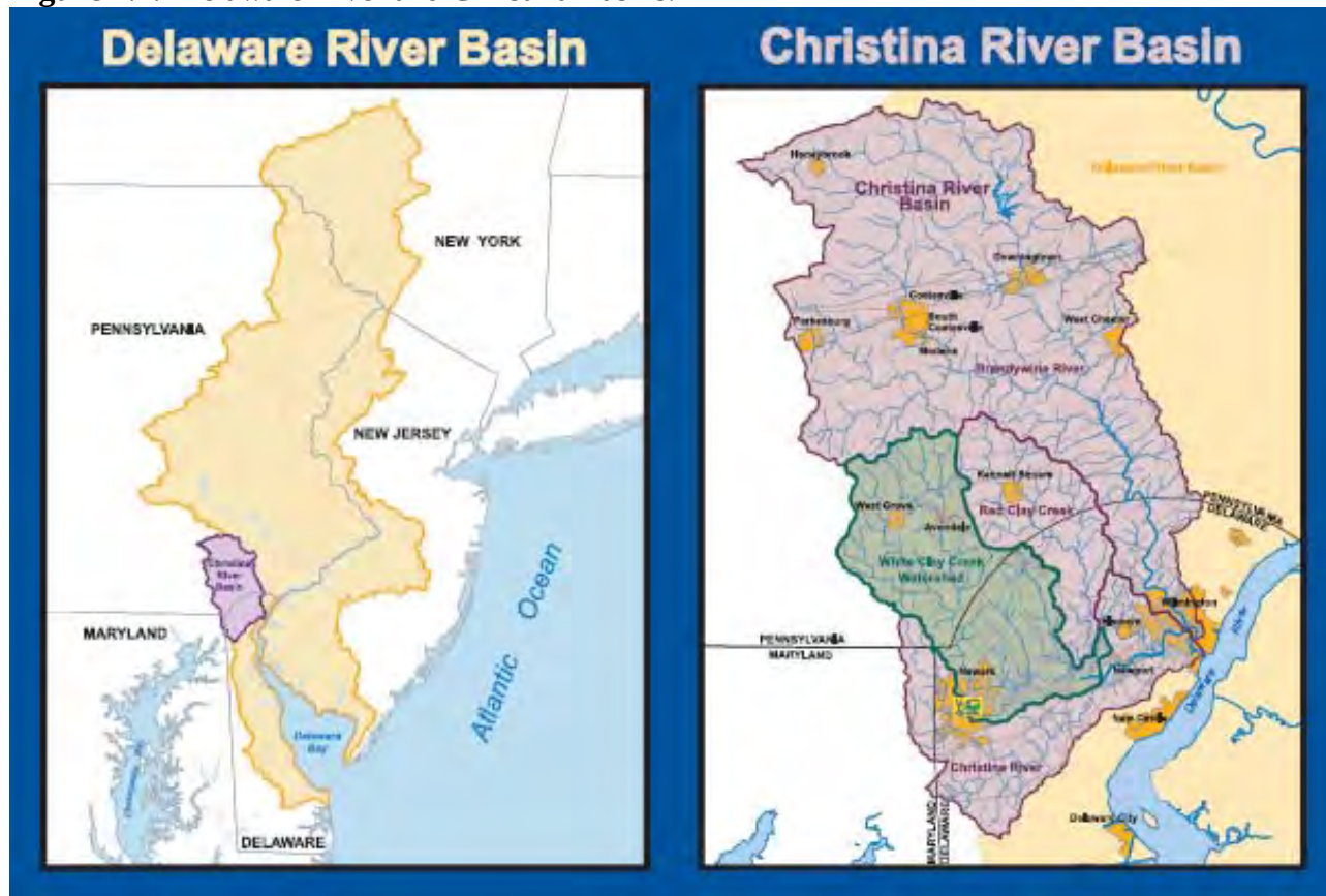
Figure 1.1. Delaware River and Christina Basins.
