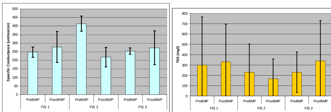
Figure A1-2. Storm-flow Specific Conductance and Total Suspended Solids at FIS1, FIS2, and FIS3. Post BMP mean Specific Conductance is less than pre BMP mean Specific Conductance at FIS2 ( p < 0.05 , one tailed test).
