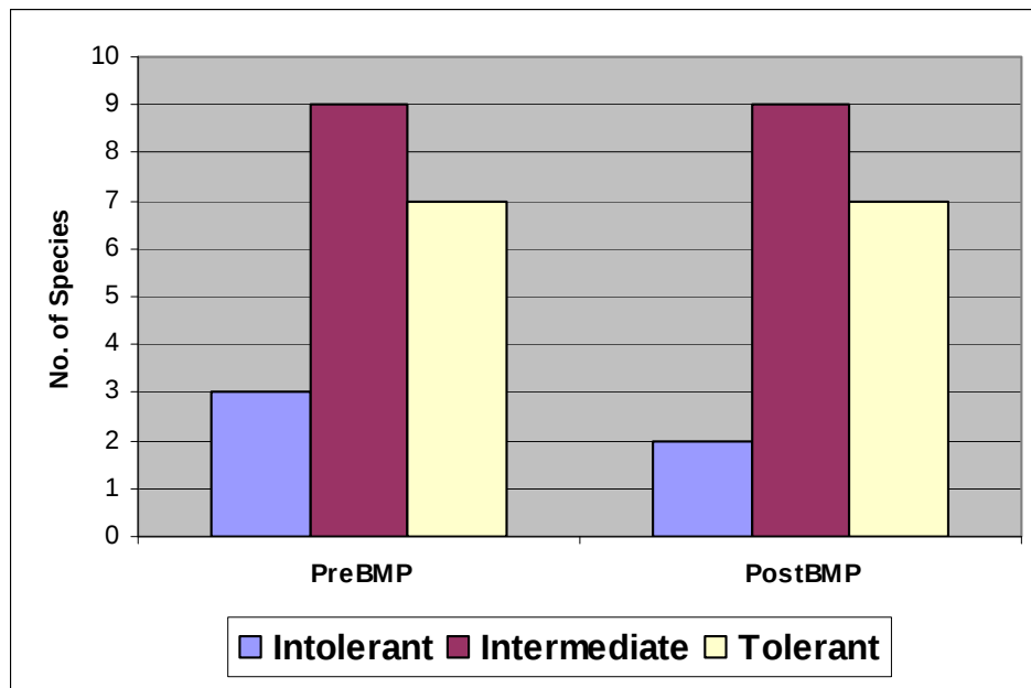
Figure 4.8. Number of fish species, pre- and post-BMP conditions.
