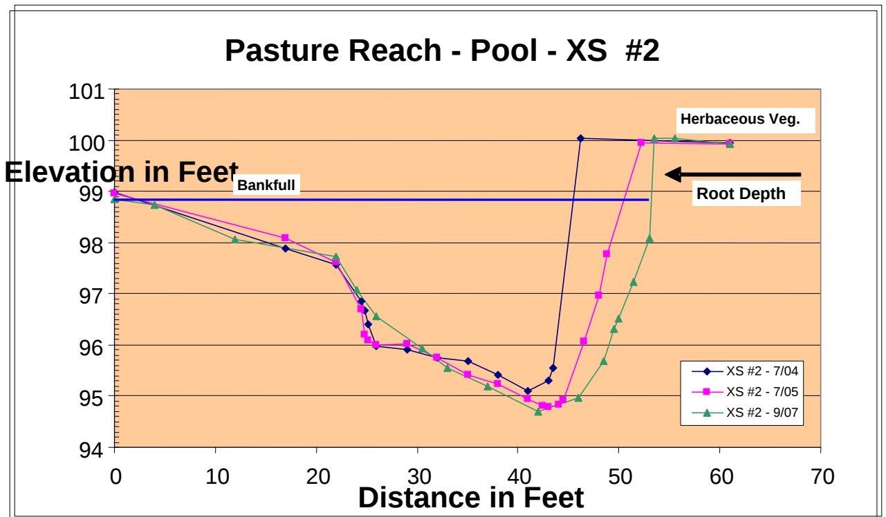
Figure 1 Pasture reach pool cross-section changes throughout study showing bankfull elevation relative to rooting depth.
