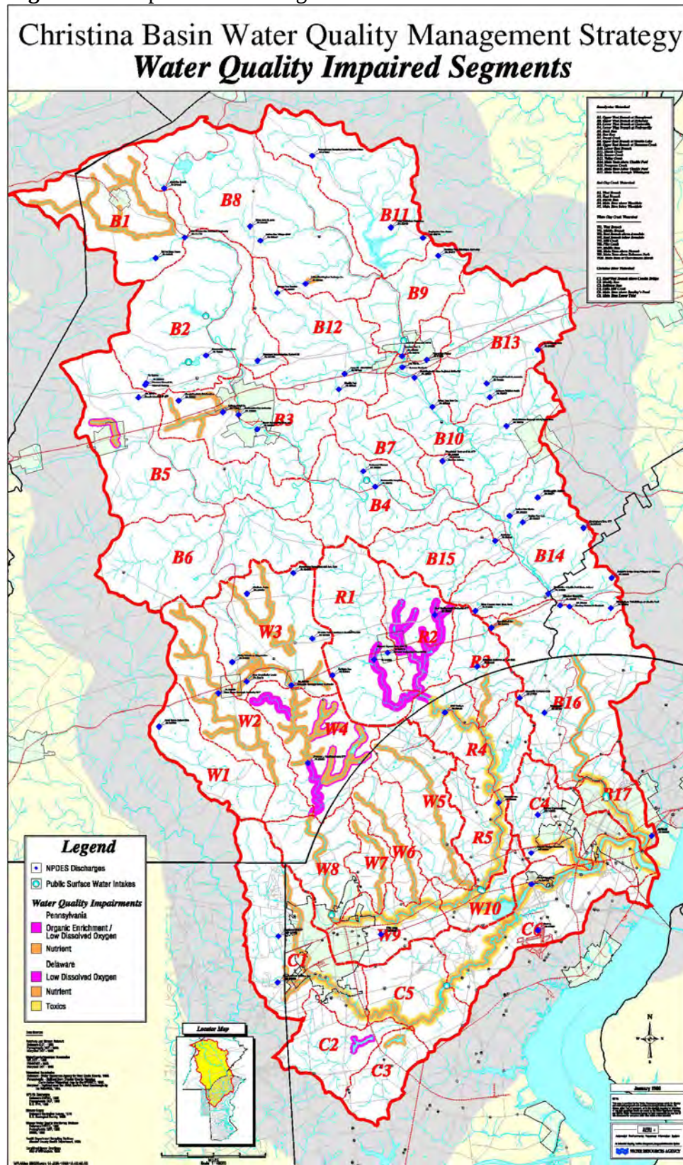
Figure 1.2. Impaired stream segments in the Christina Basin.
