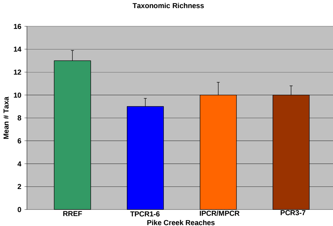
Figure 12. Mean number of taxa per unrestored and restored reaches at Pike Creek. The mean number of taxa decreased 10% one year-post restoration. The 2006 restored sites also had 10% less TR than the 2006 upstream, unrestored reaches. The 2006 regional reference is indicated in green. The blue column represents the 2006 restored reach at the Three Little Bakers Golf Course (TPCR 1-6). The orange column represents the 2006 unrestored, upstream segments at Independence School (IPCR 1-3) and Meadowdale (MPCR1). The brown column represents the 2002 unrestored reach (PCR 3-7) at the Three Little Bakers Golf Course ( \pm SE).
