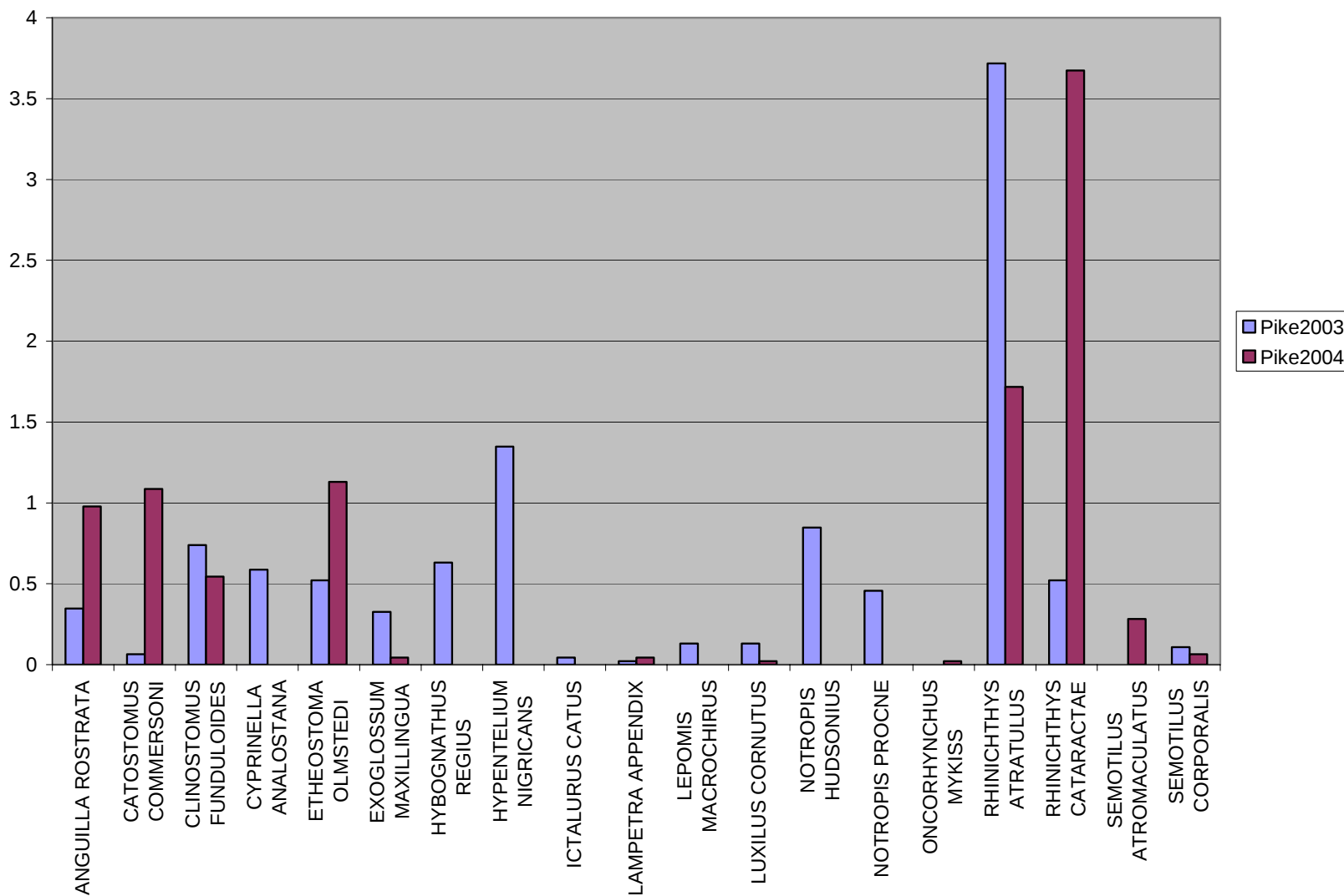
Figure 1. Fish relative abundance at the restoration site in 2004 (Pike2004) and at a survey location downstream conducted in 2003 (Pike2003).
