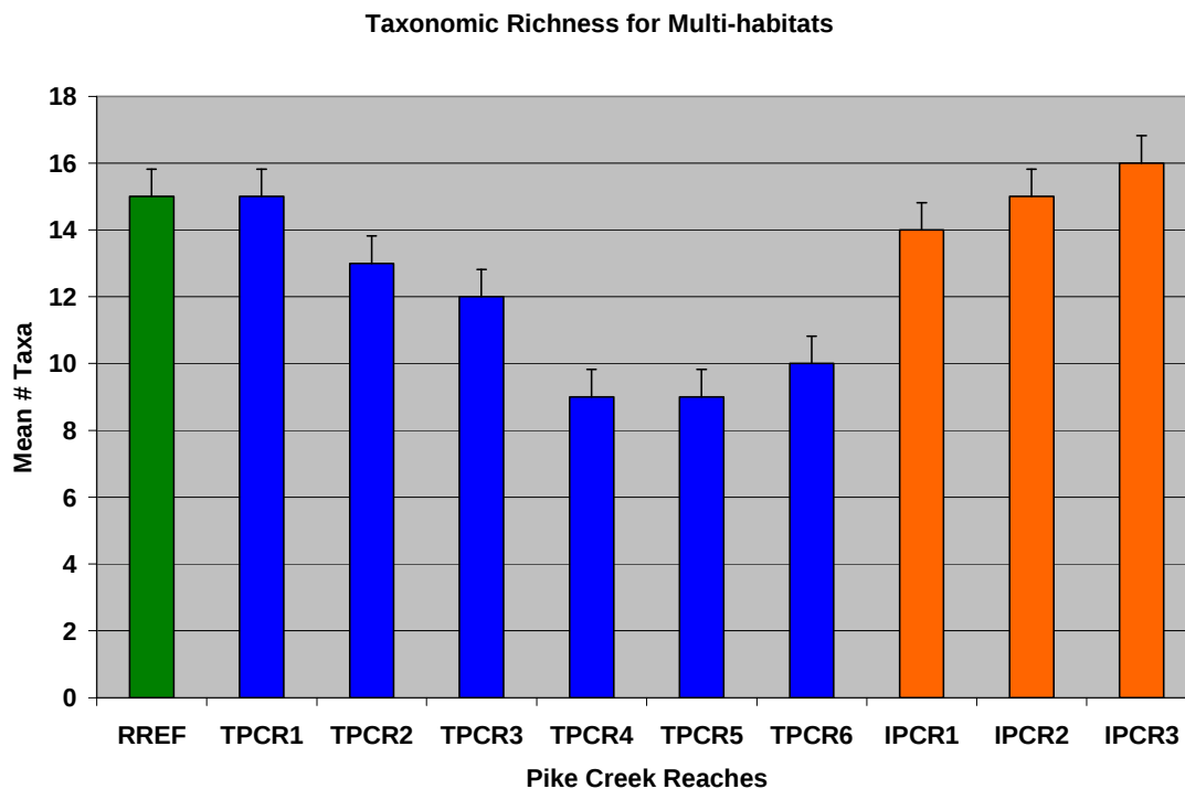
Figure 14. Mean Taxonomic Richness for multi-habitat types from Pike Creek. Taxonomic richness was less than the regional reference in the restored sites (TPCR 1-6 in blue bars) and equaled or exceeded the regional reference (RREF green bar) for the unrestored sites (IPCR 1-3, orange bars) ± SE.
