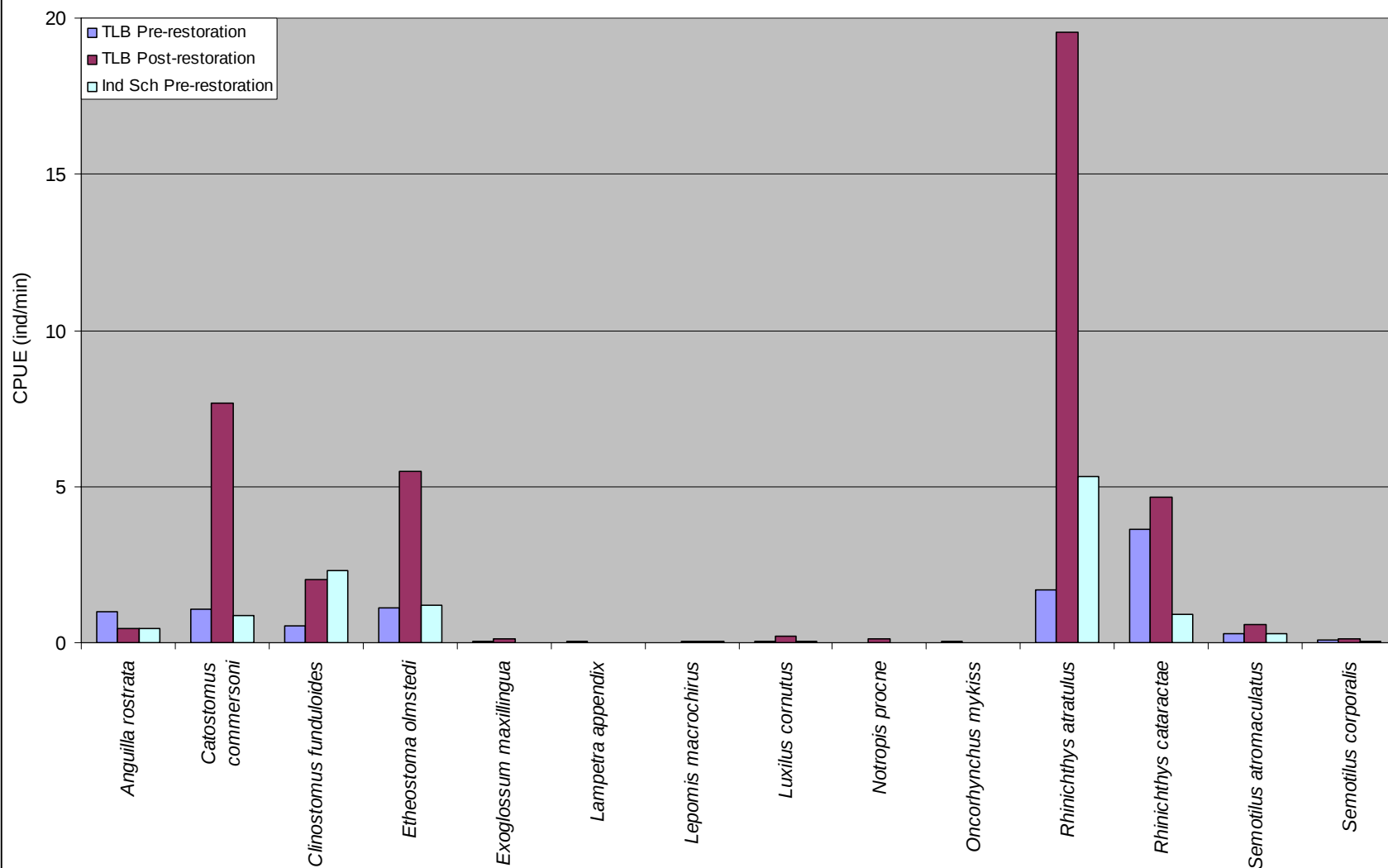
Figure 2. Fish relative abundance (CPUE) at Pike Creek restoration sites.
