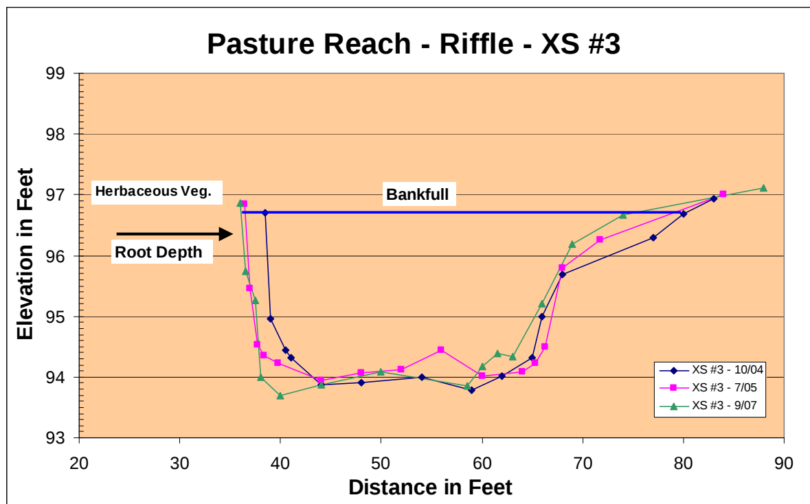
Figure A1-5. Riffle Cross-section in pasture reach.
