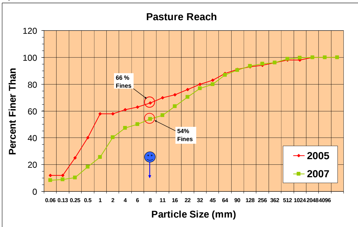
Figure 3 Stream bed particle size distribution in the pasture reach prior to (2005) and following (2007) BMP installation.
