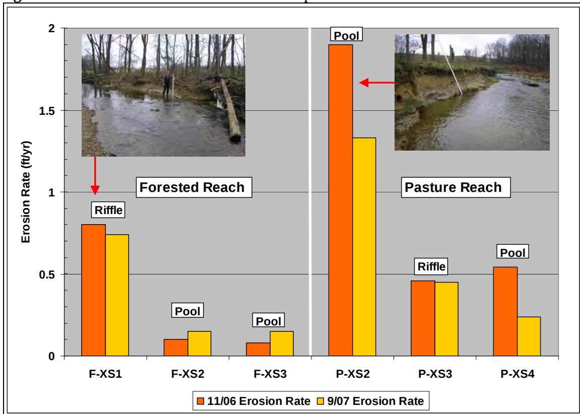
Figure 4.6. Bank erosion rates at forested and pasture reach FGM cross-sections.
