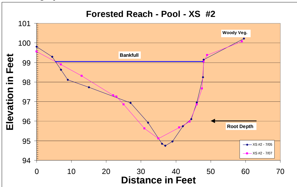
Figure 2 Forested reach pool cross-section changes throughout study showing bankfull elevation relative to rooting depth.
