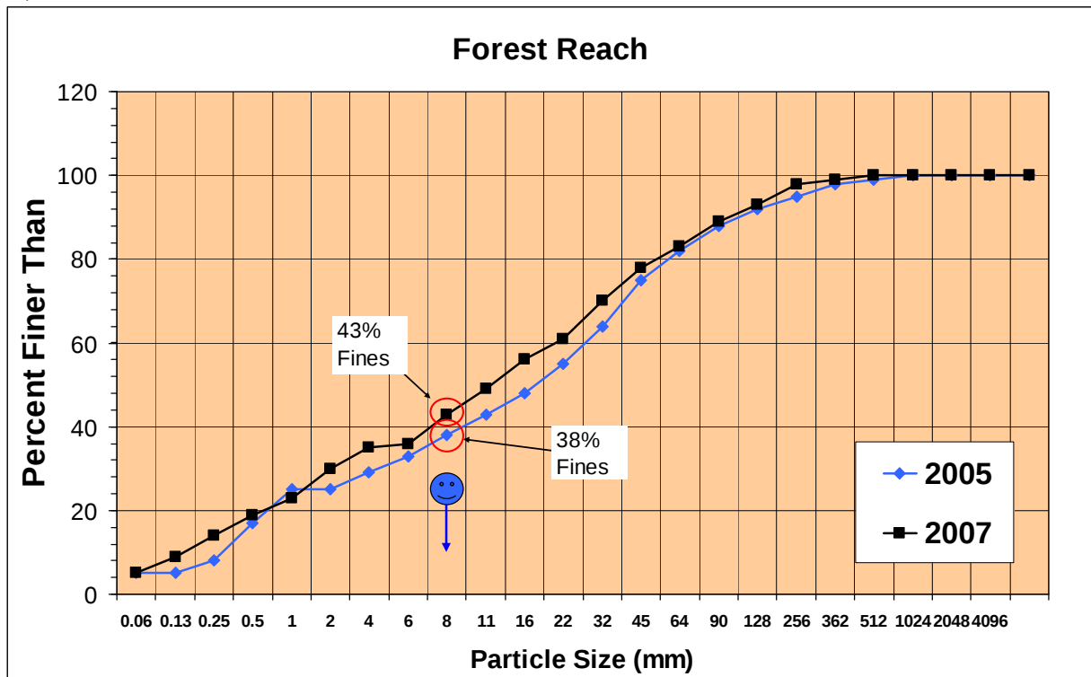
Figure 4 Stream bed particle size distribution in the forested reach prior to (2005) and following (2007) BMP installation.
