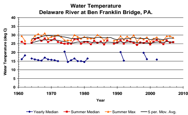
Figure 6.39. Water temperatures along the Delaware River and tributaries.
