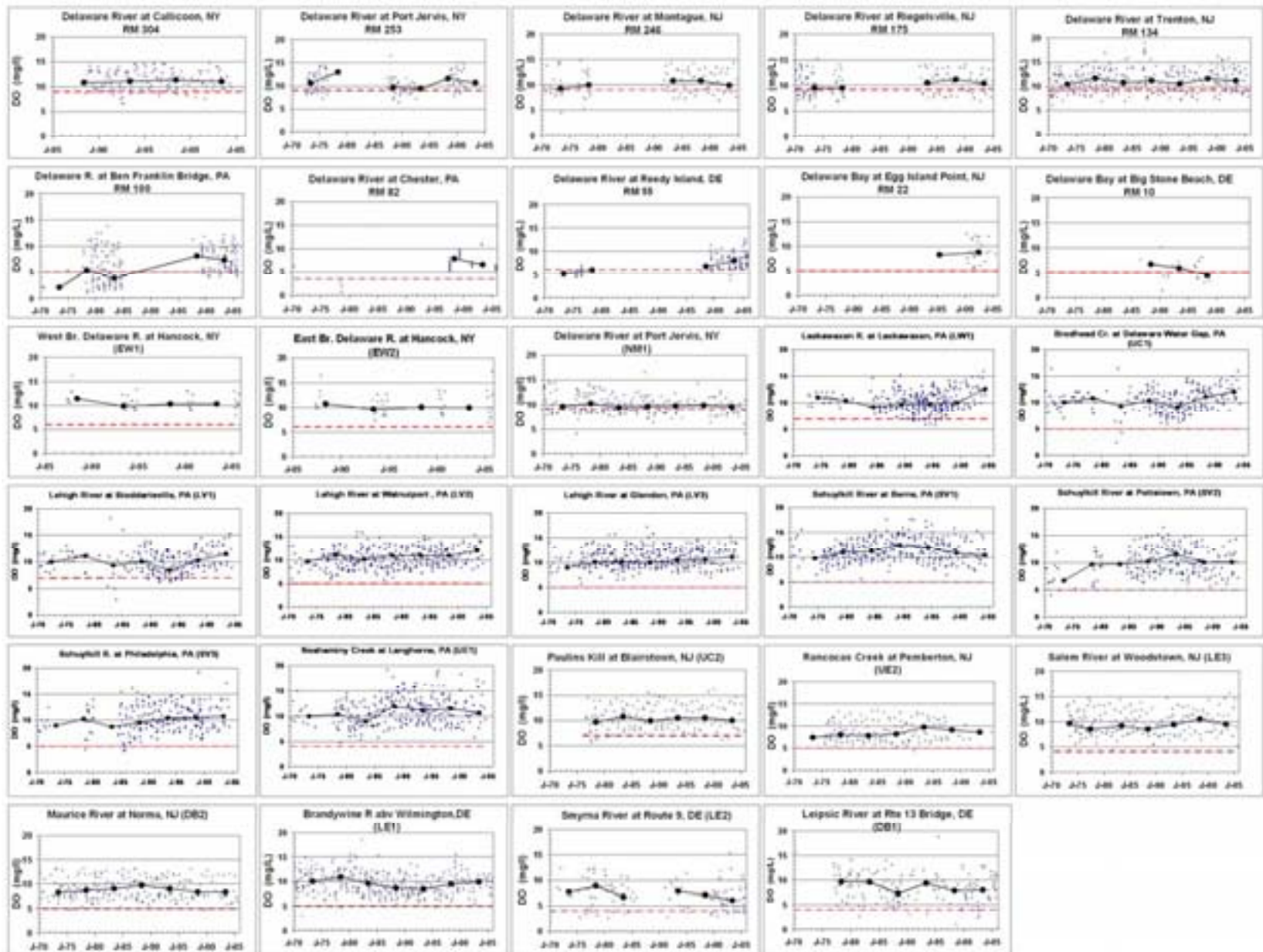
Figure 6.12. Dissolved oxygen trends in the Delaware River Basin.
