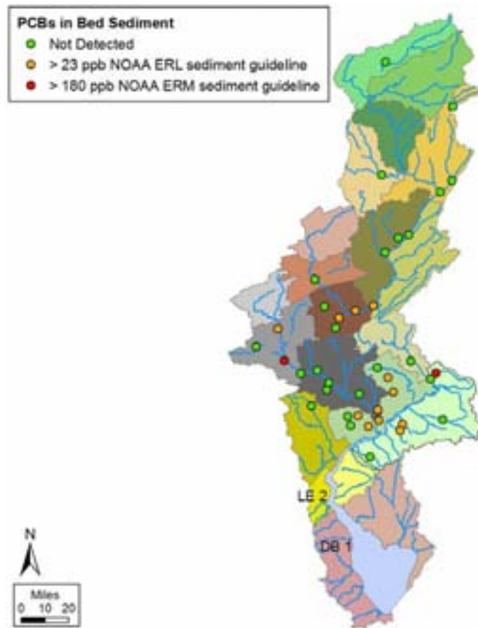
Figure 6.29. PCB in bed sediments in the Delaware River Basin. (USGS NAWQA Program)
